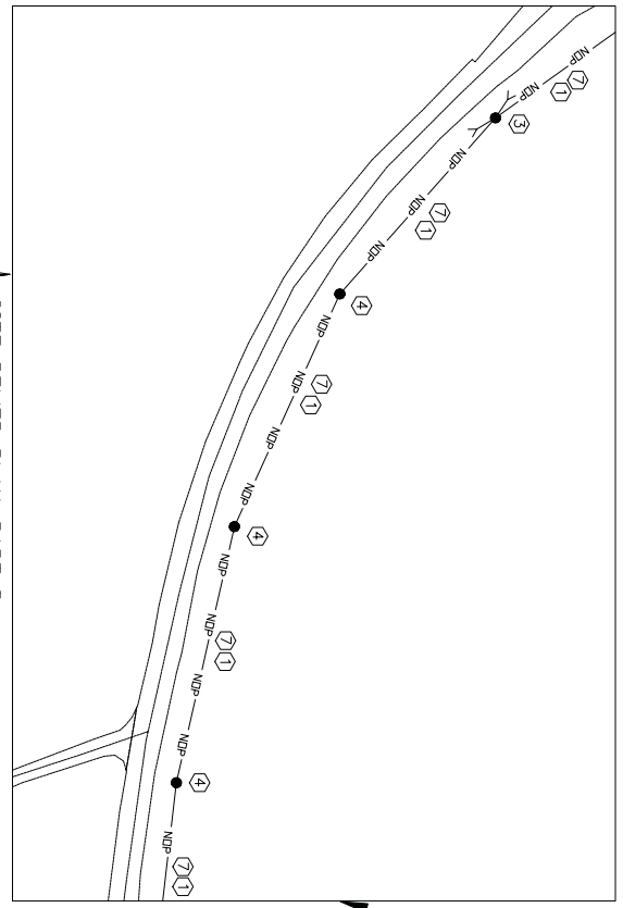
SITE POWER PLAN: PART D SCALE 1" = 40'-0"
